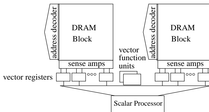
Figure 12-6 Vector IRAM Organization
