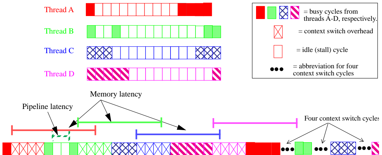
Figure 11-27 Latency tolerance in the blocked multithreading approach.
